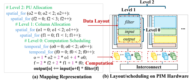
Figure 5: OptiPIM mapping representation on PIM hardware.
