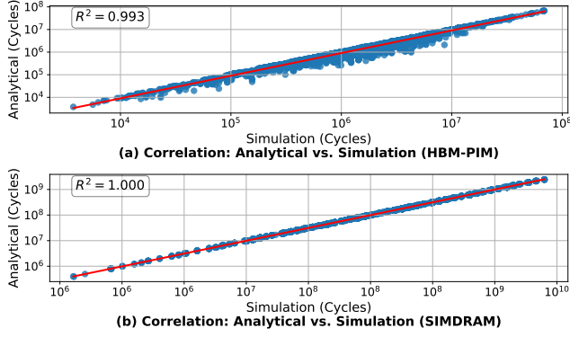
Figure 9: Validation of analytical model against Ramulator 2 [41] with PIM extension.
